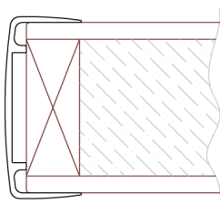
Aluminium Clashed (DE3)
