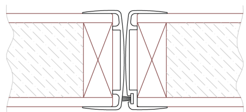
Aluminium Bullnose (DE5)
