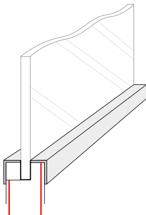
AB1-Pb Aluminium Bead Lead-Lined
