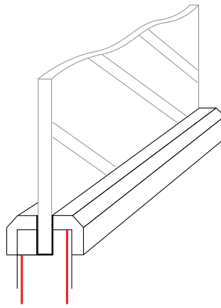
TB3-Pb Rebated Timber Lead-Lined
