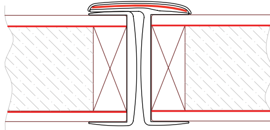
Aluminium Rebated (DE17)
