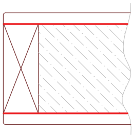
DE1-Pb Single Door Lead-Lined
